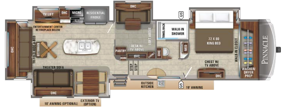
37MDQS OPTIONS: A, B, D 10' AWNING (OPTIONAL) EXTERIOR TV (OPTION)
