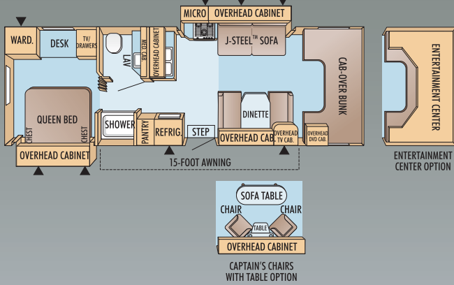
30GS Ford® E450 Chassis
