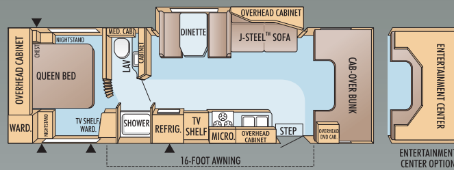
31SS Ford® E450 Chassis
